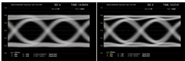
12G-SDI Source VP-P = 779.7mV
