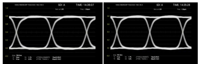
3G-SDI Source VP-P = 789.3mV
